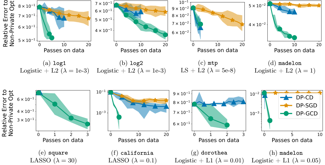
Figure 1: Relative error (min/mean/max over 10 runs) to non-private optimal for DP-GCD (our approach) versus DP-CD and DP-SGD. On the x-axis, 1 tick represents a full access to the data: p iterations of DP-CD, n iterations of DP-SGD and 1 iteration of DP-GCD. Number of iterations, clipping thresholds and step sizes are tuned simultaneously for each algorithm.
