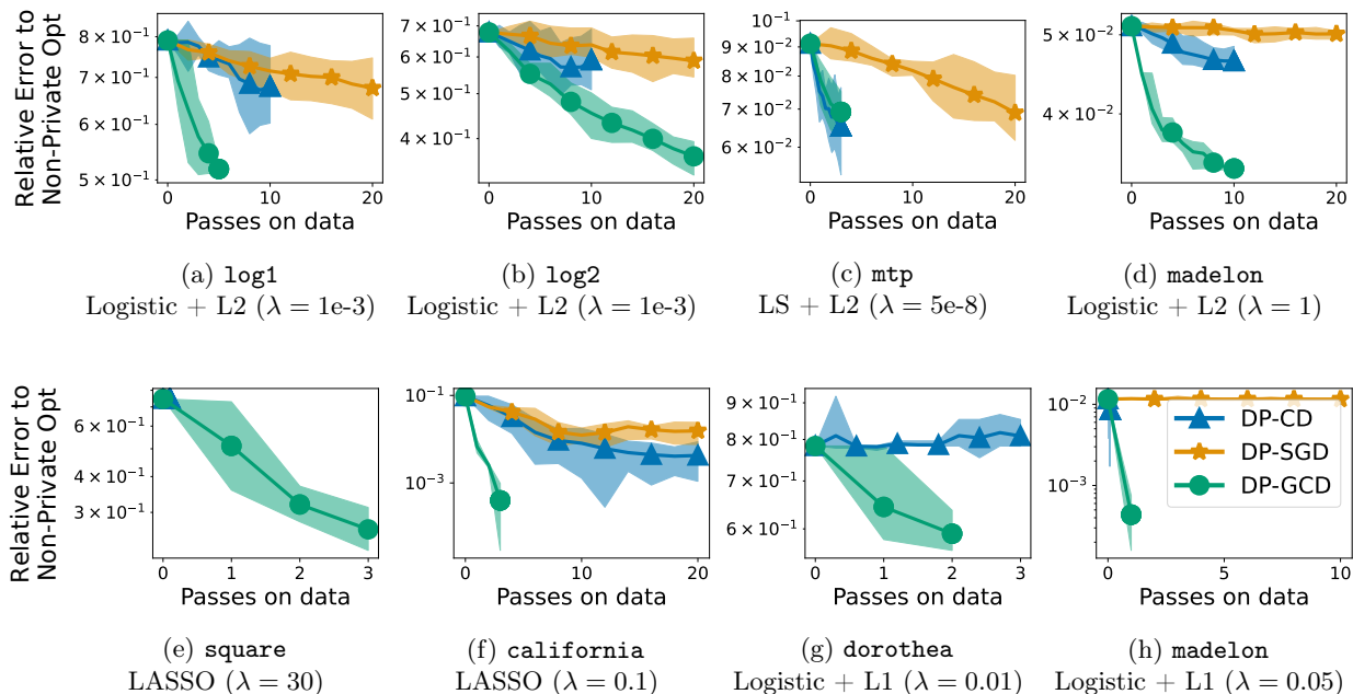
Figure 1: Relative error (min/mean/max over 10 runs) to non-private optimal for DP-GCD (our approach) versus DP-CD and DP-SGD. On the x-axis, 1 tick represents a full access to the data: p iterations of DP-CD, n iterations of DP-SGD and 1 iteration of DP-GCD. Number of iterations, clipping thresholds and step sizes are tuned simultaneously for each algorithm.
