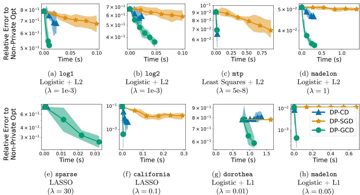
Figure 4: Relative error to non-private optimal for DP-CD, DP-GCD and DP-SGD on different problems, as a function of running time. Number of iterations, clipping thresholds and step sizes are tuned simultaneously for each algorithm. We report min/mean/max values over 10 runs.
