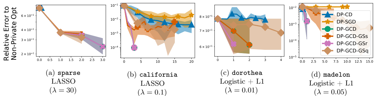
Figure 3: Relative error to non-private optimal for DP-CD, proximal DP-GCD (with GS-r, GS-s and GS-q rules) and DP-SGD on different problems. On the x-axis, 1 tick represents a full access to the data: p iterations of DP-CD, n iterations of DP-SGD and 1 iteration of DP-GCD. Number of iterations, clipping thresholds and step sizes are tuned simultaneously for each algorithm. We report min/mean/max values over 10 runs.
