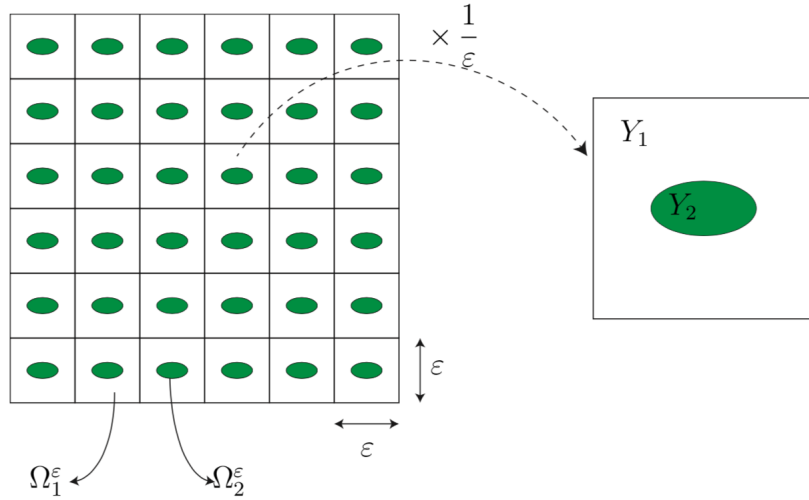
Figure 2.1: The composite periodic material and the corresponding reference cell Y .
