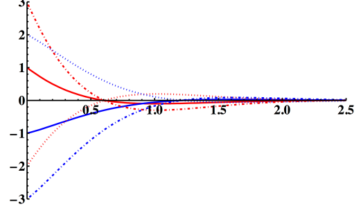
Fig. 1. Simulations of (43) Showing x_1(t) (Red) and x_2(t) (Blue) for Initial States (1, 1) (Solid), (-2, 2) (Dotted) and (3, -3) (Dashed-Dotted)
