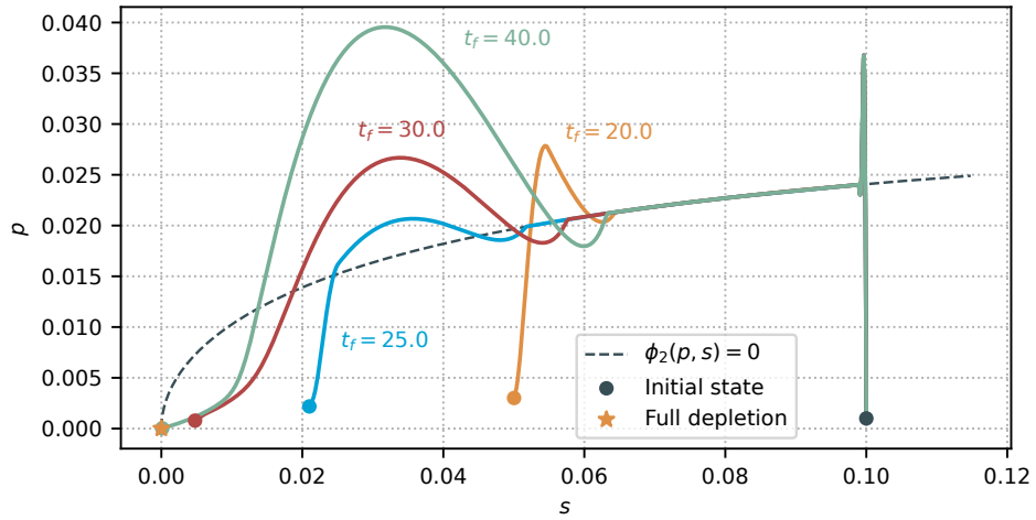
FIGURE 7. Numerical simulation of (BM-OCP) showing different trajectories in the sp -plane. Initial conditions are set to s_0 = 0.1 , p_0 = 0.001 , r_0 = 0.1 , \mathcal{V}_0 = 0.003 . In all cases, the state approaches the singular curve \phi_2 = 0 and slides along it.
