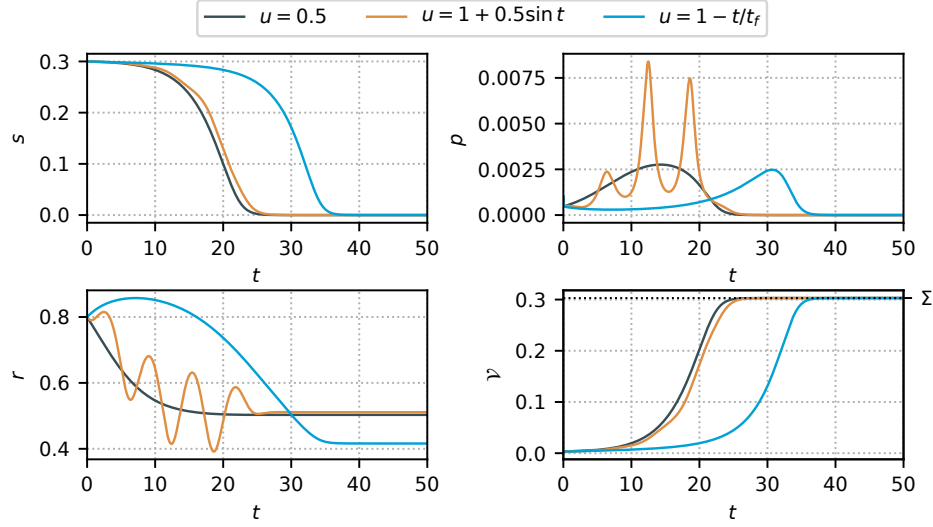
FIGURE 2. Simulation of (WTB-M) with initial conditions s_0 = 0.3 , p_0 = 0.001 , r_0 = 0.8 , \mathcal{V}_0 = 0.003 , fixed final time t_f = 50 and different allocation functions u .
