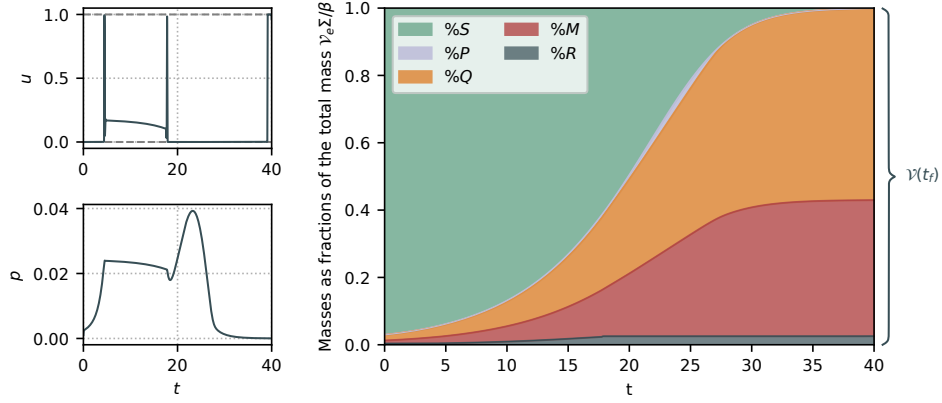
FIGURE 6. Numerical simulation of (BM-OCP) with initial conditions s_0 = 0.1 , p_0 = 0.001 , r_0 = 0.3 , \mathcal{V}_0 = 0.003 and t_f = 40 . Quantities in the right plot are shown as fractions of the total mass in the bioreactor \mathcal{V}_e \Sigma / \beta . The final volume \mathcal{V}(t_f) is at 99.8% of \mathcal{V}_e \Sigma / \beta .
