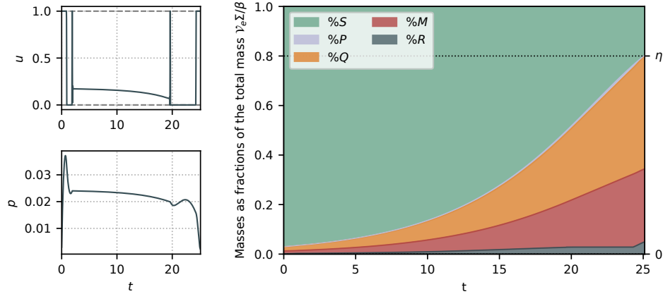
FIGURE 8. Numerical simulation of (PP-OCP) with initial conditions s_0 = 0.1 , p_0 = 0.003 , r_0 = 0.1 and \mathcal{V}_0 = 0.003 . The performance parameter is fixed to \eta = 0.8 , which is achieved in t_f = 25.1 . Quantities in the right plot are shown as fractions of the total mass in the bioreactor \mathcal{V}_e\Sigma/\beta .
