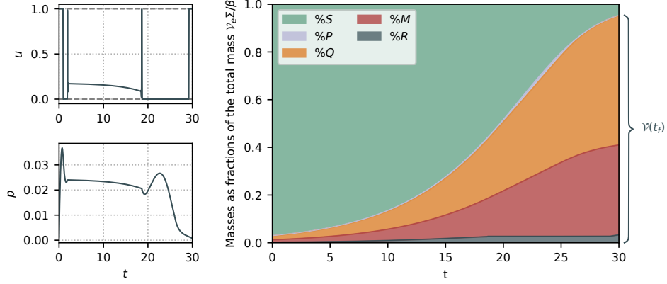
FIGURE 4. Numerical simulation of (BM-OCP) with initial conditions s_0 = 0.1 , p_0 = 0.001 , r_0 = 0.1 , \mathcal{V}_0 = 0.003 and t_f = 30 . Quantities in the right plot are shown as fractions of the total mass in the bioreactor \mathcal{V}_e \Sigma / \beta . The final volume \mathcal{V}(t_f) is at 95% of \mathcal{V}_e \Sigma / \beta .
