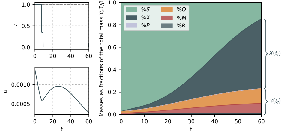
FIGURE 10. Solution of (MP-OCP) for the metabolite maximization case x(t_f) , with s_0 = 0.1 , p_0 = 0.001 , r_0 = 0.1 , \mathcal{V}_0 = 0.003 and t_f = 60 . The final product concentration x(t_f) is at 62% of the total mass in the bioreactor \mathcal{V}_e \Sigma / \beta , while the final volume \mathcal{V}(t_f) is only at 23%.
