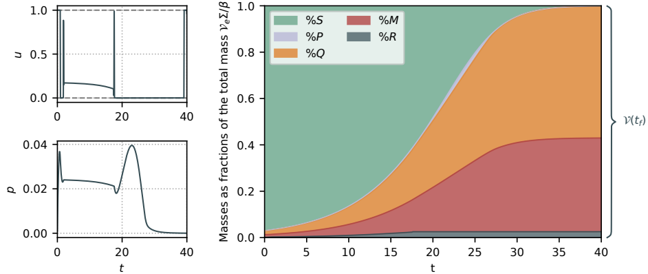
FIGURE 5. Numerical simulation of (BM-OCP) with initial conditions s_0 = 0.1 , p_0 = 0.001 , r_0 = 0.1 , \mathcal{V}_0 = 0.003 and t_f = 40 . Quantities in the right plot are shown as fractions of the total mass in the bioreactor \mathcal{V}_e \Sigma / \beta . The final volume \mathcal{V}(t_f) is at 99.8% of \mathcal{V}_e \Sigma / \beta .
