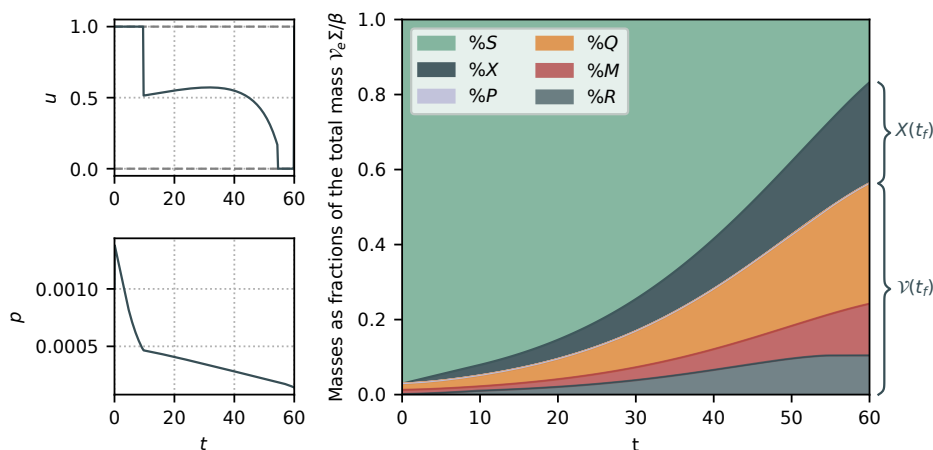
FIGURE 12. Solution of (MP-OCP) for the biomass maximization case \mathcal{V}(t_f) , with s_0 = 0.1 , p_0 = 0.001 , r_0 = 0.1 , \mathcal{V}_0 = 0.003 and t_f = 60 . The final product concentration x(t_f) is at 27% of the total mass in the bioreactor \mathcal{V}_e \Sigma / \beta , while the final volume \mathcal{V}(t_f) is at 56%.
