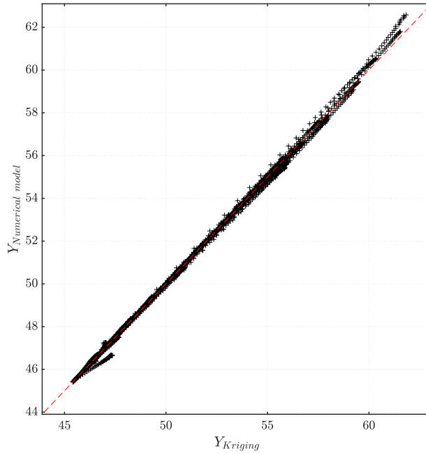
Figure 11: Plot of the values of temperatures computed by the surrogate model ( Y_{Kriging} ) against the values from the numerical model ( Y_{Numerical\ model} ), evaluated on an independent validation set of input points.
