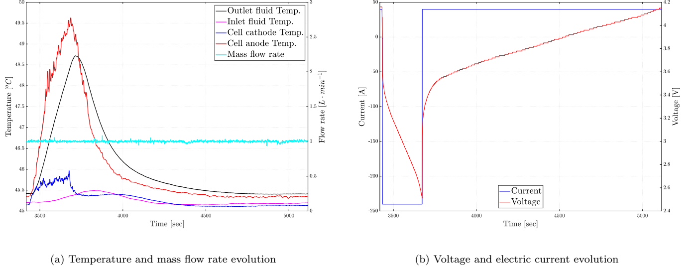
Figure 5: Experimental measurements for the Datasheet cycle.
