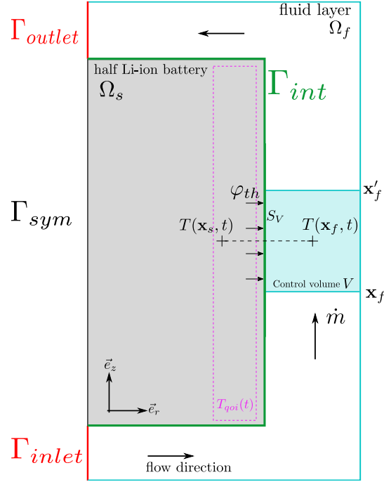
Figure 7: Computational domains: solid domain and fluid layer, control volume scheme for the specific enthalpy computation.
