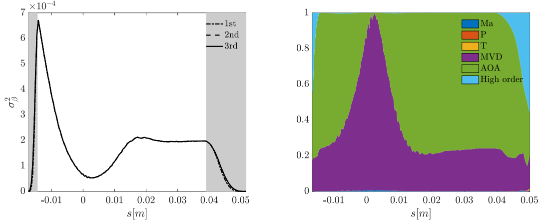
Fig. 6 Test case A. Collection efficiency ( \beta ) uncertainty analysis. (a) Collection efficiency variance for different PC truncation orders. The shaded area represents the region of the airfoil surface in to which the impingement limits are found with input parameters varying within the preset uncertainty bounds. (b) First order Sobol indexes.
