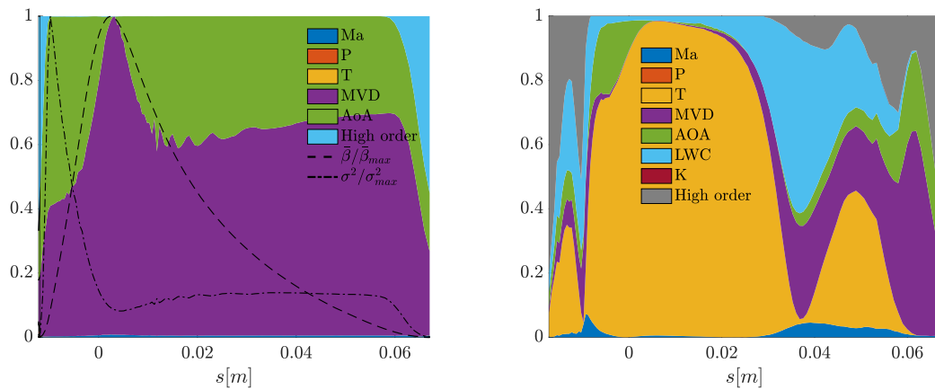
Fig. 11 Test case C. First order Sobol indices. (a) Collection efficiency \beta . (b) Ice layer thickness B .
