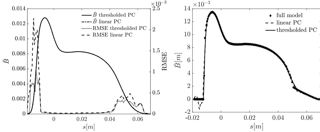
Fig. 9 Test case C. (a) Mean ice thickness and RMSE for the linear and thresholded PCE surrogates. (b) Single random PC realization. Comparison of a single PC realization, obtained for the same input, from the linear and the thresholded PC surrogates.
