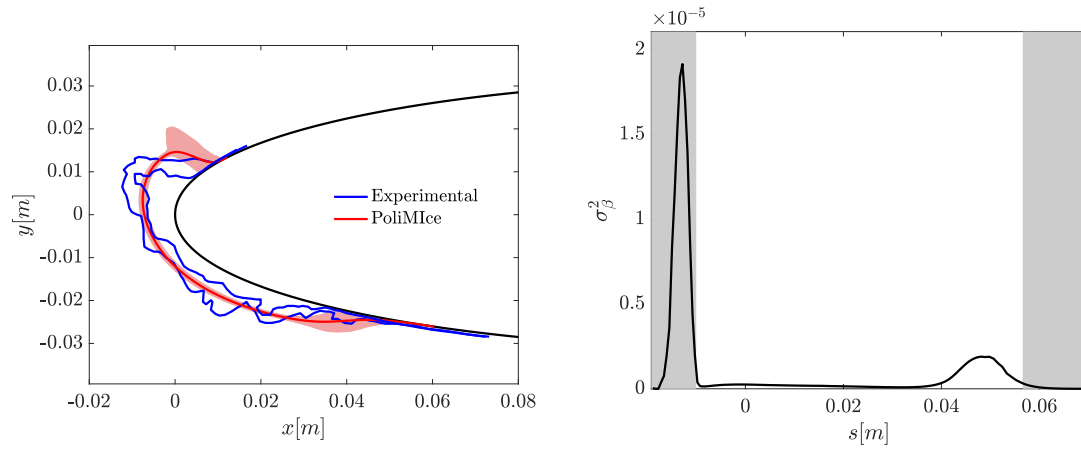
Fig. 10 Test case C. (a) Ice thickness distribution on NACA0012 airfoil. Computed and experimental bounds. (b) Ice thickness variance w.r.t. the curvilinear abscissa. The shaded area represents the region of the airfoil surface in to which the ice accretion limits are found with input parameters varying within the preset uncertainty bounds.
