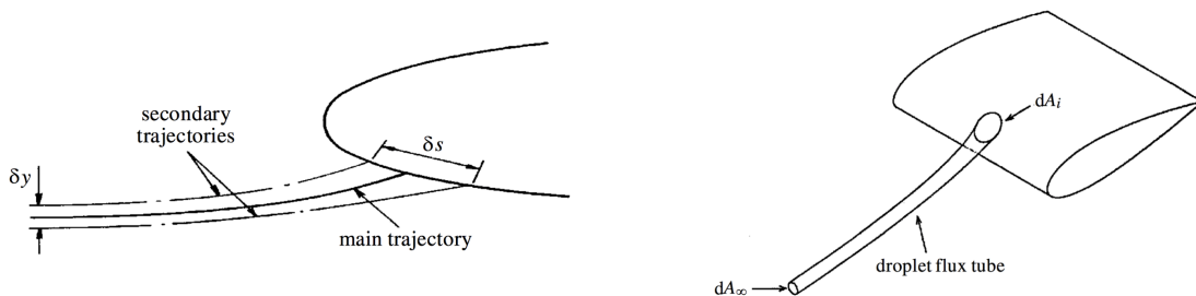
Fig. 3 Collection efficiency parameter \beta computed for a two and a three-dimensional problem, from Ref. [16]
