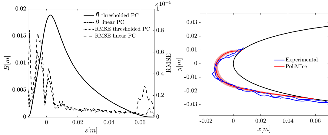
Fig. 7 Test case B. (a) Mean ice thickness and RMSE for the linear and thresholded PCE surrogates for the rime case. (b) Comparison between experimental data and computed ice shape for the NACA0012 rime case.
