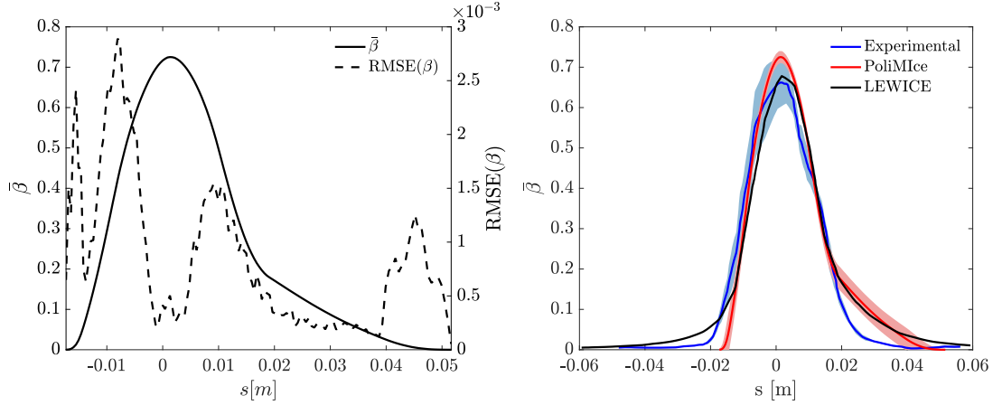
Fig. 5 Test case A. Collection efficiency ( \beta ) surrogate assessment. (a) Mean \beta (left scale) and RMSE (right scale) of PC predictions evaluated on the test set. (b) Comparison among numerical predictions and experimental observations. Curves are complemented by the 2\sigma uncertainty obtained from PC of the computational model and experiment repeatability studies.
