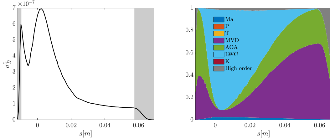
Fig. 8 Test case B. (a) Ice thickness variance w.r.t. the curvilinear abscissa. The shaded area represents the region of the airfoil surface in to which the ice accretion limits are found with input parameters varying within the preset uncertainty bounds. (b) First order Sobol indexes.
