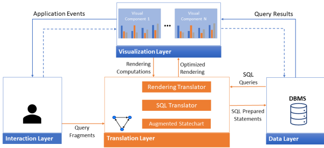
Figure 1: The interaction-driven framework for big data exploration (the translation layer is highlighted in orange).
