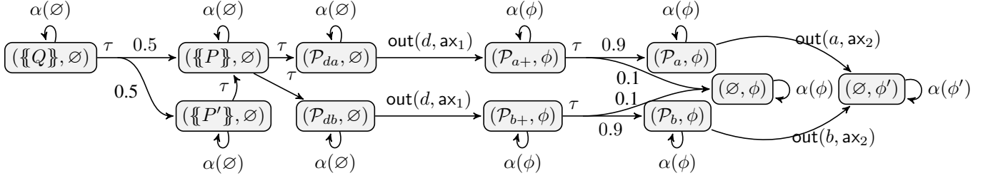
(a) The fragment of N^l corresponding to (\{Q\}, \emptyset) and (\{P\}, \emptyset)
