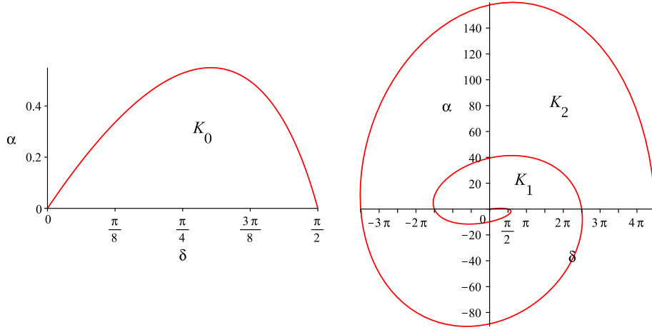
Fig. 3.1: Left: stability region in terms of the parameters \alpha and \delta . Right: the spiral (3.3) represented for y \in [0, \frac{9\pi}{2}] ; note that the stability region K_0 of the left panel is barely visible in the display of the right panel.
