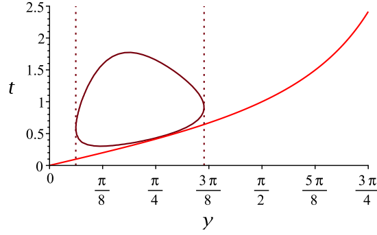
Fig. 5.1: Representation of K(x, t) = 0 and t = \tan(y/2) for arbitrary parameter values \alpha = 0.074 , \beta = 0.45 and \gamma = 0.235 , chosen so that the curves are tangent. The vertical dotted lines mark the bounds (5.3).
