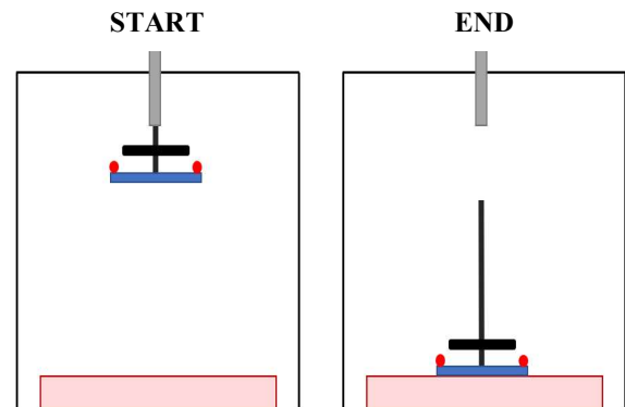
Figure 1: The impactor. The markers (red circles) placed at the four corners of the squared base (blue rectangle) were used to define the center of the impact surface. The 10kg mass (black rectangle). Rod to guide (black vertical line) and mat (red base).
