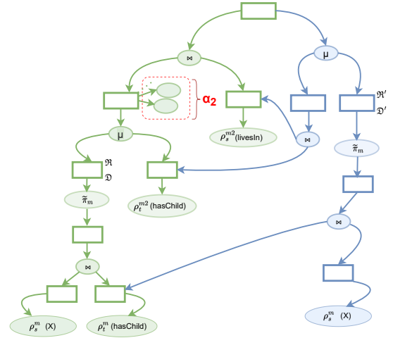
Figure 11: Expansion of a RLQDAG by pushing a join in a fixpoint operation node. The initial RLQDAG is in green color, and parts added by pj() are in blue color.
