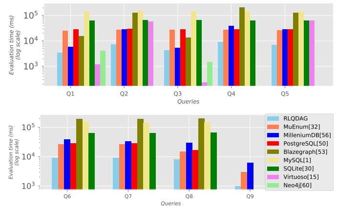
Figure 25: Comparative evaluation of third-party queries (excerpt from [54]).
