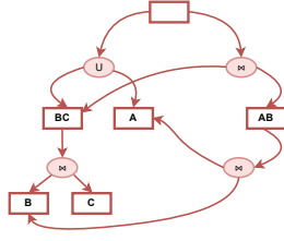
Figure 6: Not well-formed RLQDAG.
