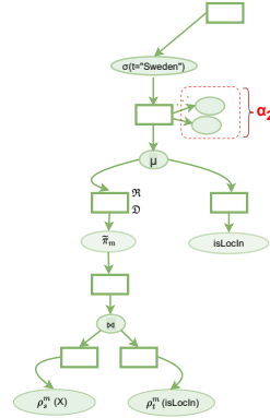
Figure 8: Initial RLQDAG before expansion with opportunity to apply pf() .
