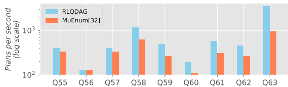
Figure 20: Non-regular queries.
