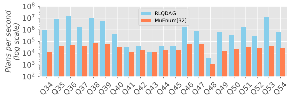
Figure 19: Airbnb and LDBC queries.
