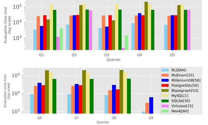
Figure 25: Comparative evaluation of third-party queries (excerpt from [54]).
