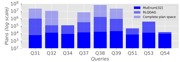
Figure 21: Plan spaces explored in 500ms.
