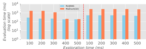
Figure 24: Evaluating best estimated plans found in explored spaces of Fig 22.
