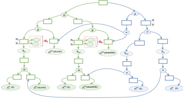
Figure 13: RLQDAG structure after merging fixpoint operation nodes.
