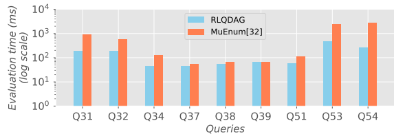
Figure 23: Evaluating best estimated plans found in explored spaces of Fig 21.
