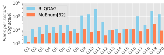
Figure 17: Yago queries.
