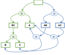
Figure 5: Well-formed RLQDAG.
