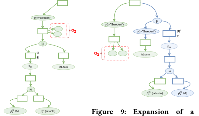
Figure 9: Expansion of a RLQDAG by pushing a filter in a fixpoint operation node, with branches added by pf() in blue color.
