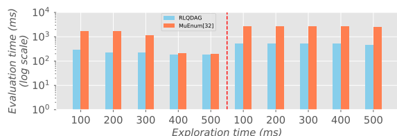
Figure 24: Evaluating best estimated plans found in explored spaces of Fig 22.
