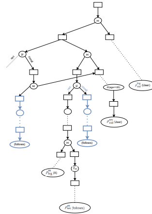
Fig. 5: Another tree branch creation.
