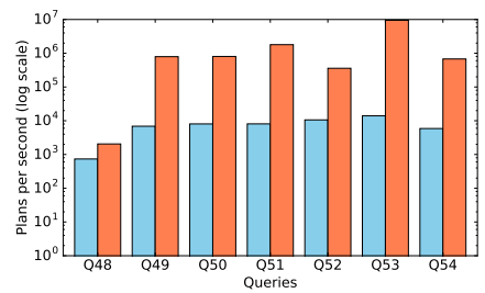
Fig. 12: LDBC queries.
