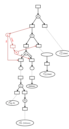
Fig. 8: Final unification.
