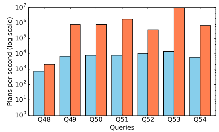
Fig. 12: LDBC queries.
