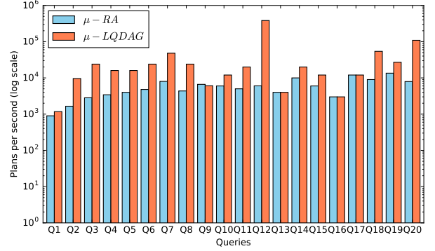
Fig. 9: Yago queries.
