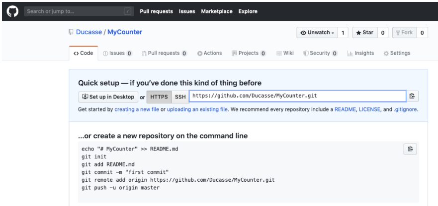
Figure 5-16 GitHub HTTPS address our project.
