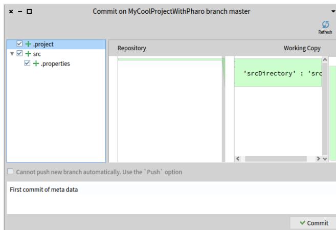
Figure 7-13 Details of metadata commit.
