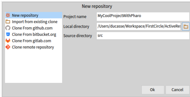
Figure 7-19 Creating a local repository without pre-existing remote repository.
