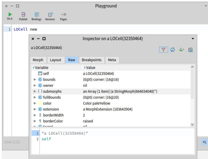
Figure 6-8 The inspector used to examine a LCell object.
