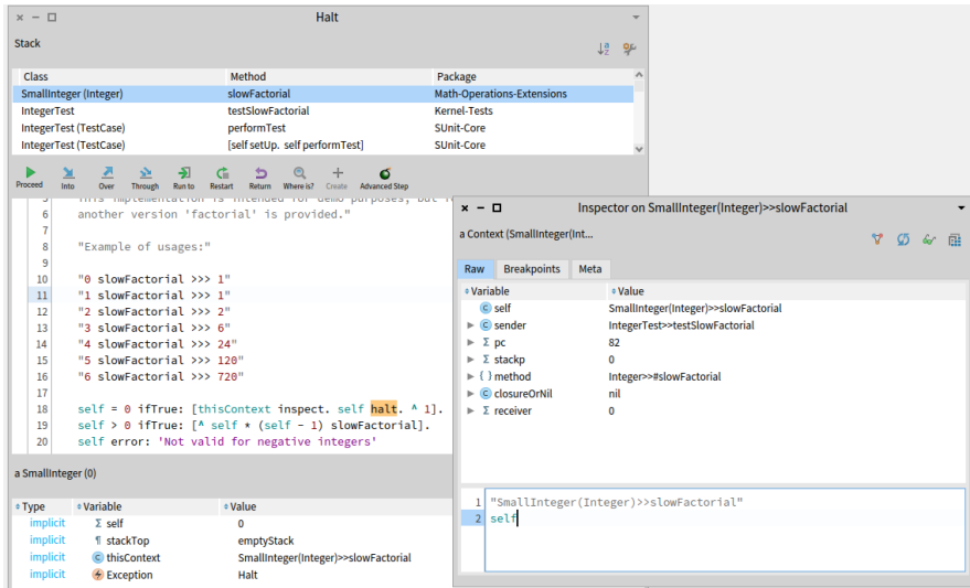
Figure 18-7 Inspecting thisContext.
