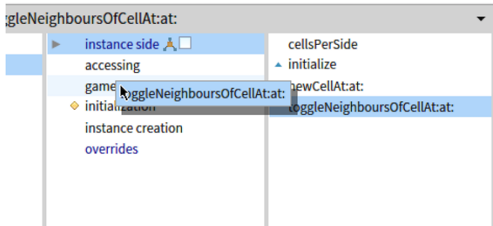
Figure 6-19 Drag a method to a protocol.
