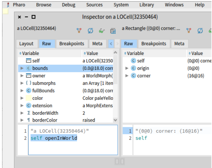
Figure 6-10 A LCell opened in the World.
