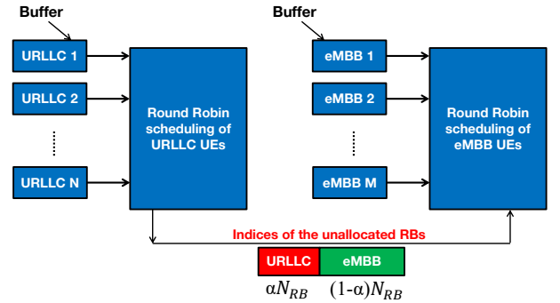
Figure 1: Scheduling strategy of URLLC and eMBB traffic
