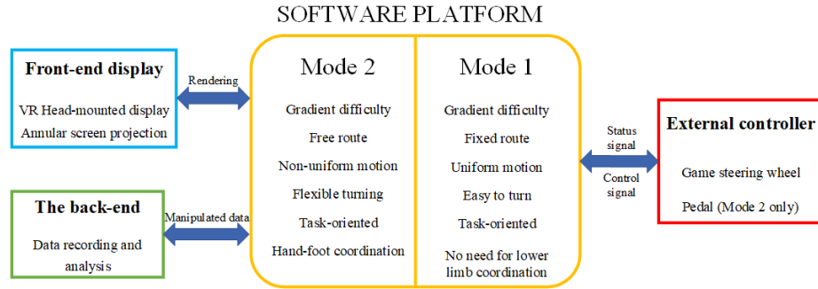
Fig. 1. Structure of VR-DLR.
