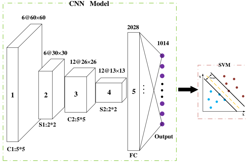
Fig. 8. CNN model in the proposed method
