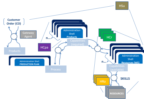
Figure 1. Proposal Framework orchestrating AAS.
