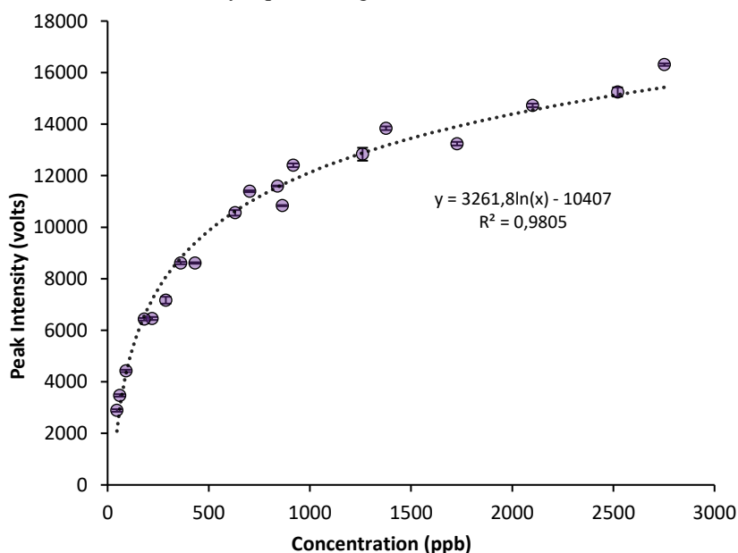
Fig. 2. Logarithmic regression for peak intensity (volts) per concentration (ppb).
