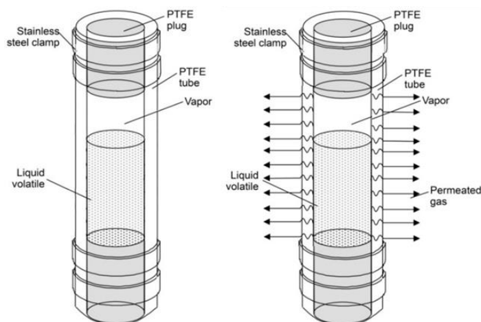
Fig. 1. A generalize schematic of permeation tubes including its components [18].
