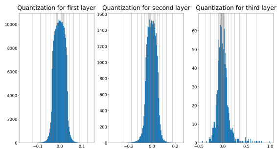
Fig. 5: Quantization indices for m = 2 and \ell = -1 .
