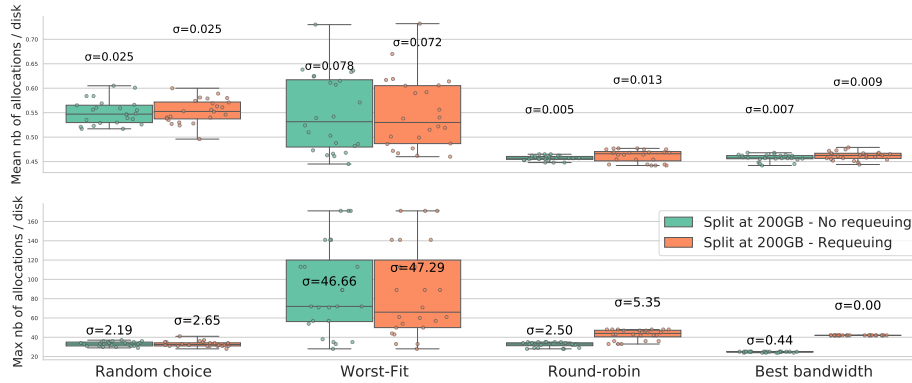
Fig. 4. Mean (top) and max (bottom) number of allocations per disk, grouped by algorithms, for 16TB platform and split strategy. Storage layout 1N1D excluded. Dots plot the mean and max number of allocations of each disk separately.
