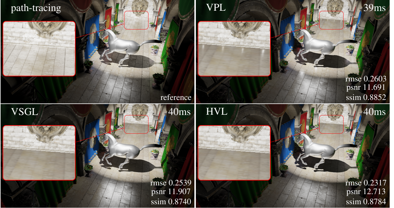
Figure 12: Comparison with 900 VPL, 529 VSGL and 400 HVL, generated at equal time. Images are rendered at 1600 \times 900 . The HVL cache resolution is 322^2 pixels, and 14^2 pixels for one VSGL. The contribution of HVLs is on 15 SH bands. In this rendering, HVL are limited to circularly symmetric specular lobe to compute lighting only on ZH. Insets show VPL spike artifacts and VSGL or HVL robustness to those artifacts. See additional material for more comparisons and implementation details.
