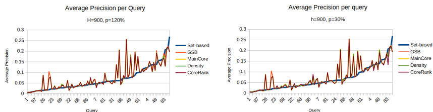
Fig. 5. Difference with Set-based Model
