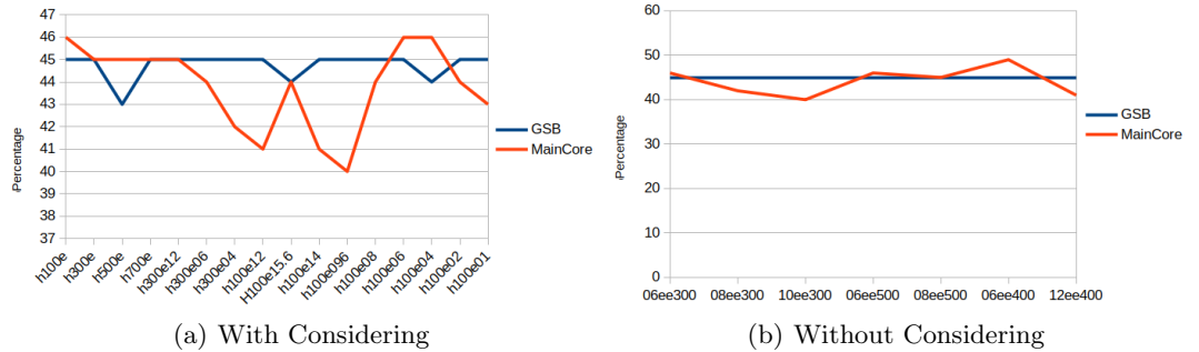
Fig. 2. Amplification on Important Nodes-Edges
