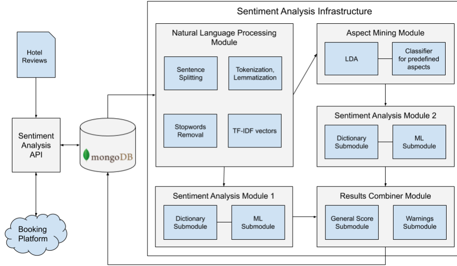
Fig. 1. Hotel Reviews Sentiment Analysis Platform Architecture
