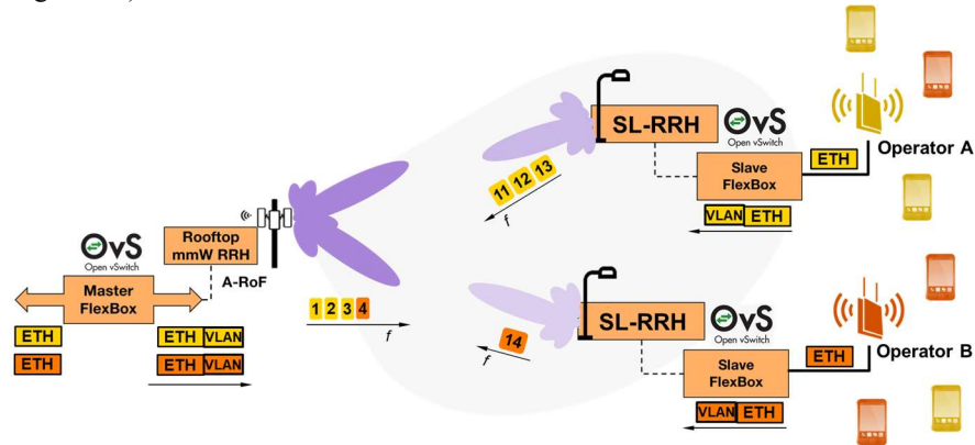
Fig. 6. 5G-PHOS multi-operator architectural instantiation using different SL-RRHs.
