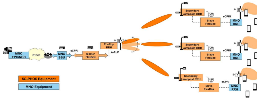
Fig. 2. The 5G-PHOS PtMP fronthaul solution for Dense Area Use Case.
