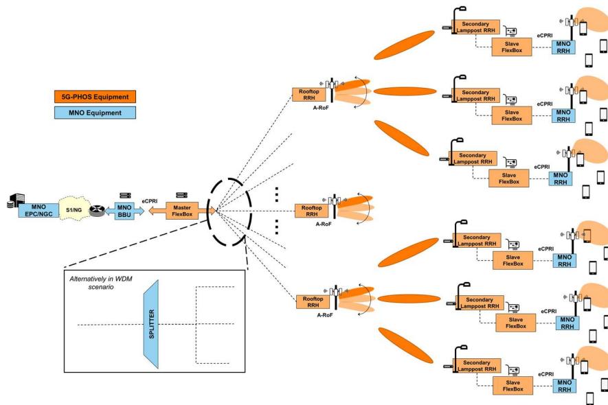
Fig. 3. The 5G-PHOS PtMP fronthaul solution in the Ultra-Dense Use Case.
