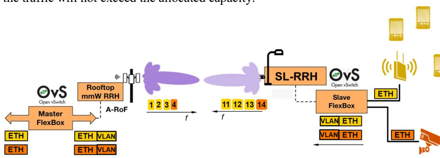
Fig. 7. 5G-PHOS multi-tenancy architectural instantiation using the same SL-RRH.
