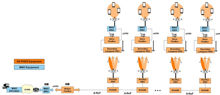
Fig. 4. The 5G-PHOS PtMP fronthaul solution in the Hotspot area Use Case.
