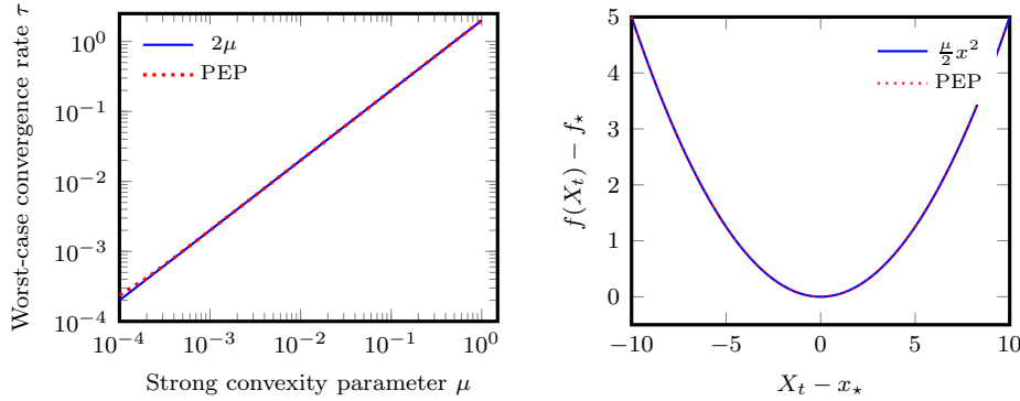
(a) Worst-case rate \tau_* for the class of quadratic Lyapunov functions (2.2)
