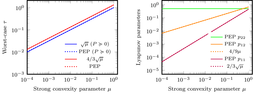
(a) Best guarantees found within the class of quadratic Lyapunov functions (2.11).
