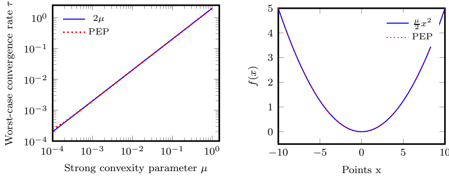
(a) Worst-case rate \tau on the class of quadratic Lyapunov functions for the gradient flow. (b) Reconstruction of a function f \in \mathcal{F}_\mu that interpolates x_0 and X_t , while matching the convergence rate \tau = -2\mu , with \mu = 0.1
