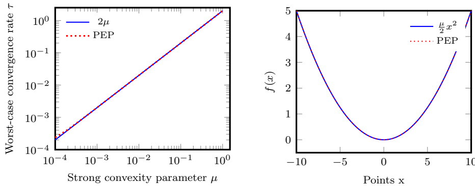
(a) Worst-case rate \tau on the class of quadratic Lyapunov functions for the gradient flow.
