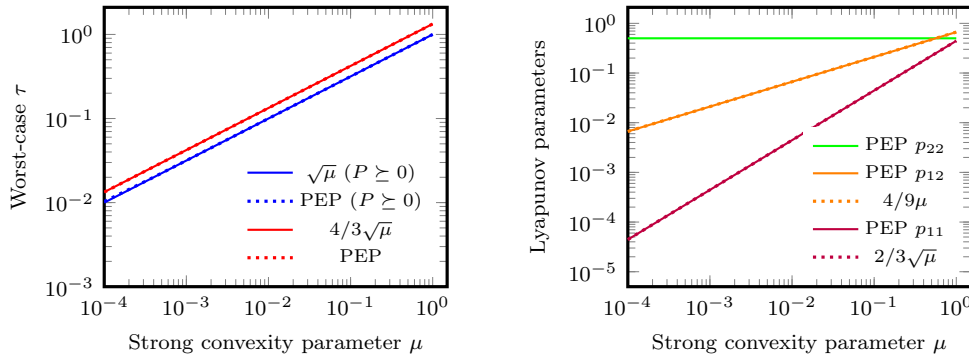
(a) Worst-case guarantee optimized over the class of quadratic Lyapunov functions. (b) Lyapunov parameters P for \tau = 4/3\sqrt{\mu} and a = 1 , as a function of the condition number \mu .
