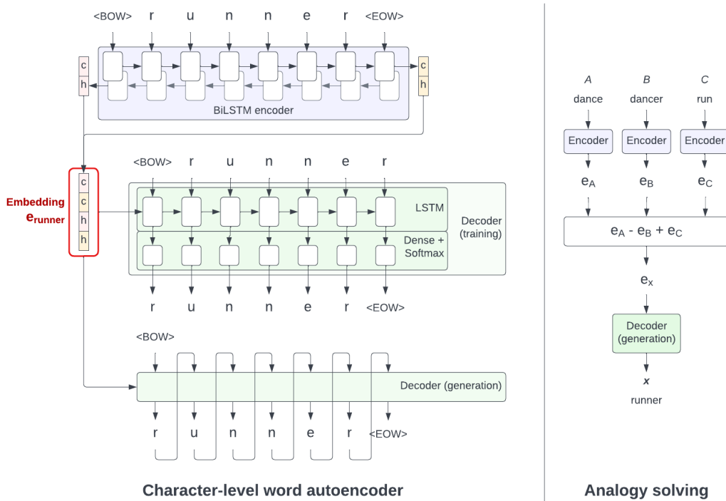
Figure 1: Character-based word auto encoder and vector arithmetic to solve analogies
