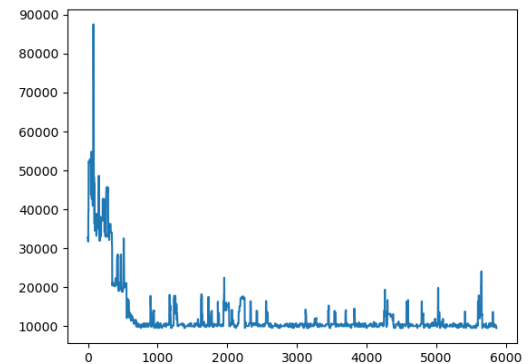
(c) Evolution of the WCET estimate when the first x option are taken (optimization sequence SO3 of size 6000).
