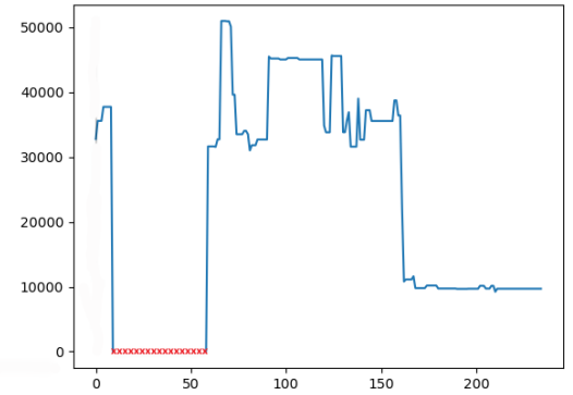
(a) Evolution of the WCET estimate when only the first x options are taken (optimization sequence SO1 of size 250).
