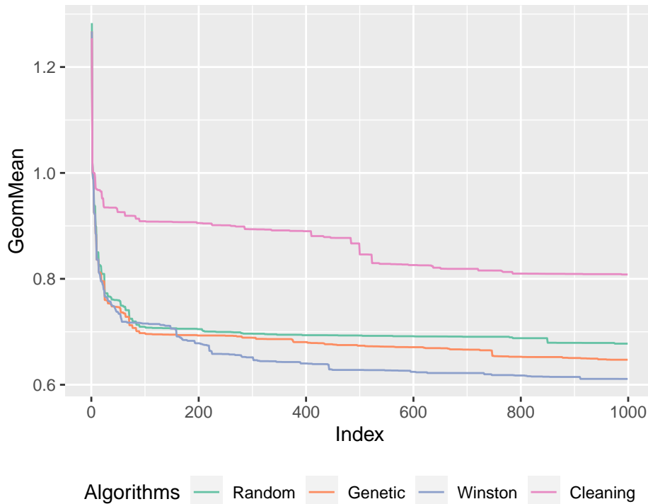
Figure 4: Result of Winston, against various algorithms of the state-of-the-art [7]. A geometrical mean over the benchmarks is used to represent the ratio between the estimated WCET, with the technique under consideration, over the estimated WCET with the best optimization level applicable (-O0..-O3).
