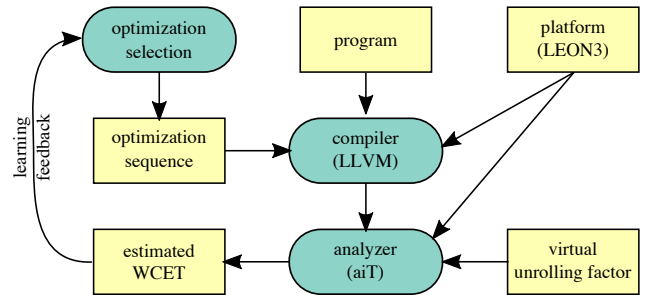
Figure 1: Iterative WCET-oriented compilation workflow (from [7])
