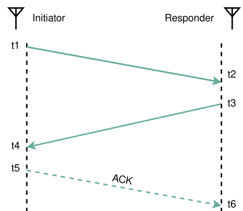
FIGURE 2. Time of Flight technique.
