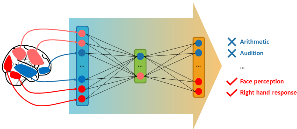
Figure 7. Explored "NNuD" models. As inputs we used the brain components loadings for the studied contrasts ( in this example "clicking when viewing a face" vs "viewing something else" ). The hidden layers were used to increase the expressive power of the model by adding non-linearities and regularize it by controlling their width. We explored networks with 0 to 3 hidden layers. The output layer scores each considered label.
