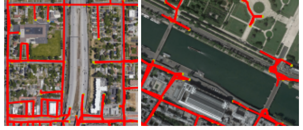
Figure 8. Examples of long sections of road without points of interest, which are occasionally missed by our method.
