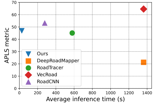
Figure 6. APLS metric with respect to inference time for our method, compared to state-of-the-art approaches. Our method is the fastest and offers a very good compromise between accuracy and speed.
