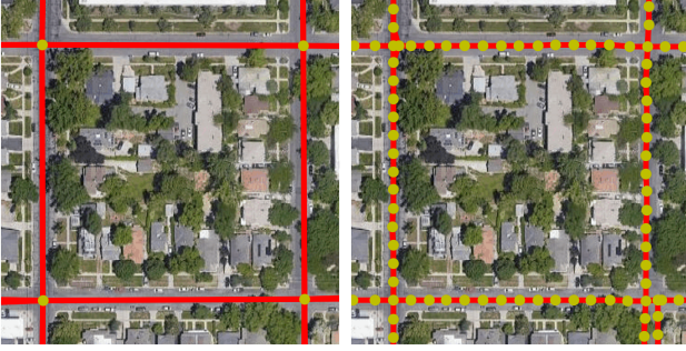
Figure 7. Example of the low complexity of the graphs inferred by our method (left) compared to VecRoad [36] (right). Our method finds an optimal 4-node representation of this simple neighborhood, whereas iterative methods tend to find overly complex representations. Having graphs with a low number of elements will save storage and speed up the computation of algorithms performed on these graphs, such as shortest path algorithms.
