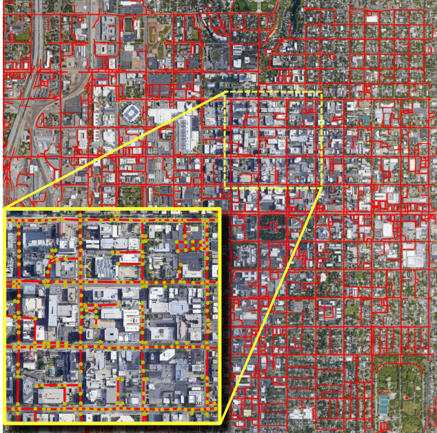
Figure 1. Result of our method on an image from the RoadTracer [3] test set. Our method regresses an entire graph without the need of pre or post-processing. This 8192x8192 pixel image was processed in 22 seconds on a single GPU, which is up to 91 times faster than previous approaches. The extracted graphs have a low complexity and retain good accuracy compared to existing works.
