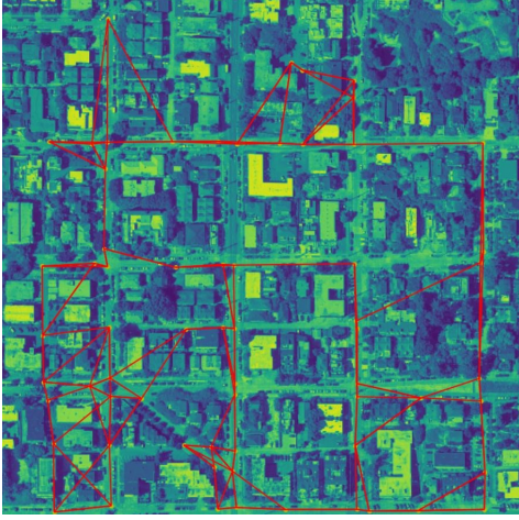
Figure 3. k = 4 -NN graph constructed in feature space on features learned by an additional node features head combined with an MLP edge classifier.
