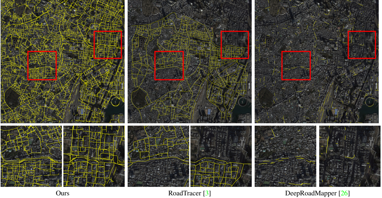
Figure 4. Comparison of our method against an iterative method [3] and a segmentation based method [26] on a challenging area of the RoadTracer dataset. The first line is the full image. The second line shows crops of the regions in red squares. Our method is able to find more roads, even in sections that are completely missed by other methods.
