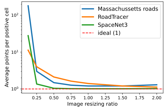
Figure 5. Average ground truth points per positive output cell at a range of image resizing ratios for 3 popular road extraction datasets. The ideal average is one, to prevent the collapse of neighboring nodes as much as possible.
