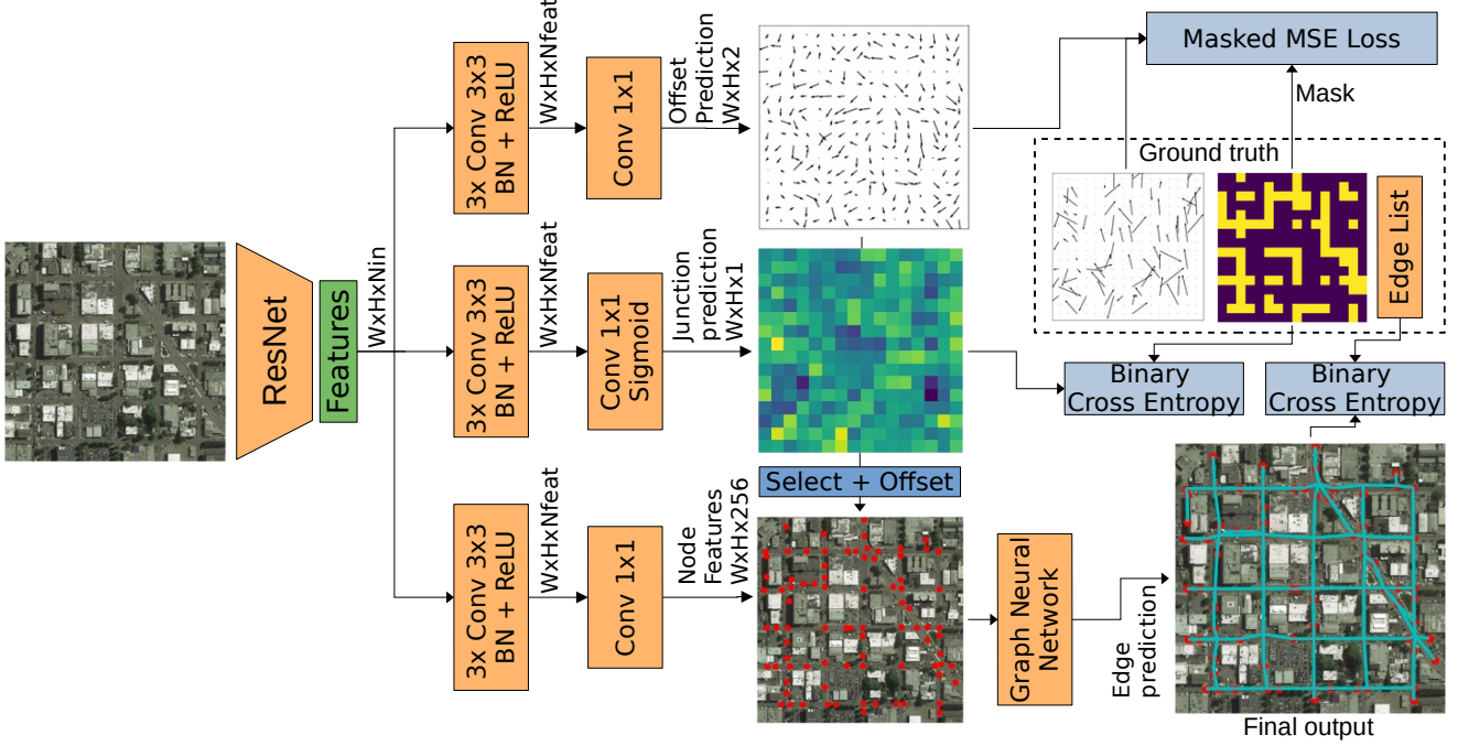
Figure 2. Our single-shot road graph extraction neural network. Features computed using a ResNet [12] backbone are fed to three branches. The junction prediction branch identifies cells which contain points of interest and is trained with binary cross-entropy. The offset prediction branch regresses the precise location of these points inside of the cells by outputting a two-dimensional vector field and is trained with a Mean Squared Error loss. Points selected by the junction and offset branch are paired with node features from a third branch and fed to a Graph Neural Network which predicts the presence of edges between pairs of points to create the final output.
