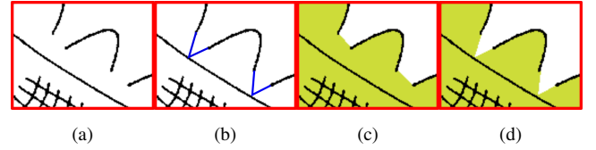
Figure 8: Sharp corners: (a) Input sketch, (b) Expected result, (c) Result of Delaunay coloring, (d) Result after gap filling procedure.
