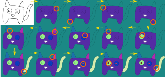
Figure 13: Various steps in the automatic segmentation algorithm. The order is shown using yellow color arrows, segmenting edges are shown in red color, the edge under consideration is marked using orange color circle.
