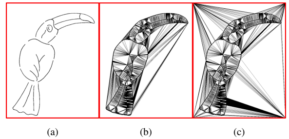
Figure 3: (a) Input sketch, (b) Delaunay triangulation of extracted sketch pixel positions, (c) Delaunay triangulation after padding points.
