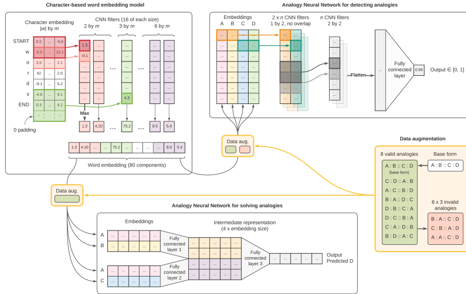
Fig. 1: Morphological embedding model, data augmentation, analogy classification (ANNC) and analogy retrieval (ANNr) models.
