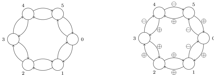
Fig. 1. Left: interaction digraph G_6^{\text{ECA}} of the ECA rule 128 for n = 6 , with local functions f_i(x) = x_{i-1} \wedge x_i \wedge x_{i+1} for all i \in \{0, \dots, 5\} . Right: update digraph corresponding to the update schedules \Delta = (\{1, 2, 3\}, \{0, 4\}, \{5\}) and \Delta' = (\{1, 2, 3\}, \{0\}, \{4\}, \{5\}) , which are therefore equivalent ( \Delta \equiv \Delta' ). For example, f^{(\Delta)}(111011) = 110000 whereas for the synchronous update schedule we have f^{(\Delta^{\text{sync}})}(111011) = 110001 .
