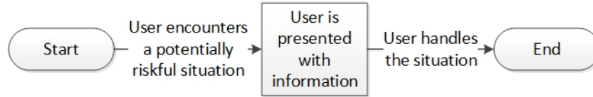
Fig. 2. CBMT overview
