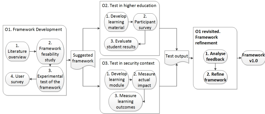
Fig. 1. Research process
