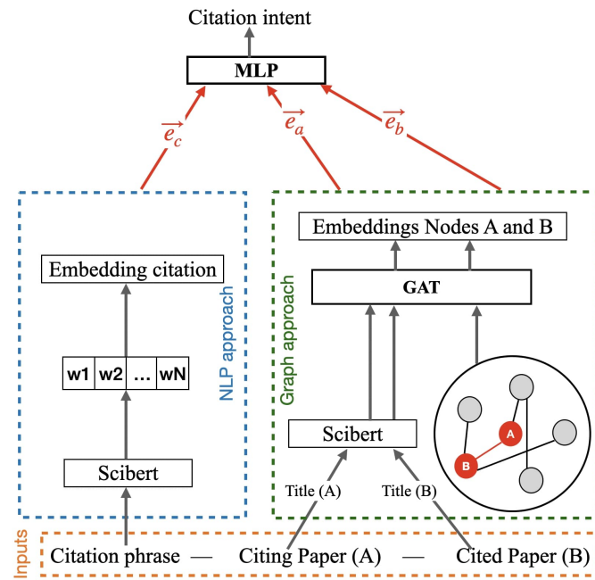
Figure 3: GraphCite
