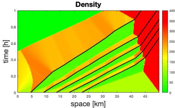
Fig. 6: Traffic density with MPC on a fleet of 5 CAVs
