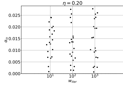
(a) \eta = 0.2
