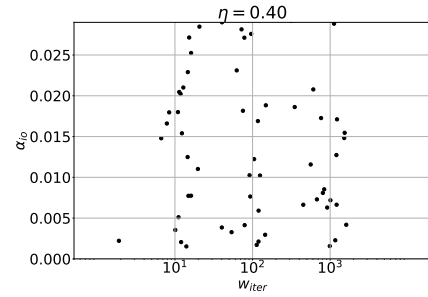
(b) \eta = 0.4
