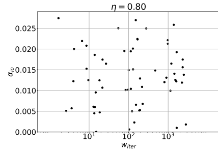
(c) \eta = 0.8
