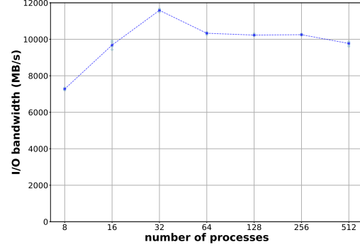
Figure 16: Average write bandwidth (from five runs) measured with IOR for different numbers of processes. In each run, eight nodes are used to write a total of 32 GB to a BeeGFS file system, using 1 MB requests and the file-per-process strategy.
