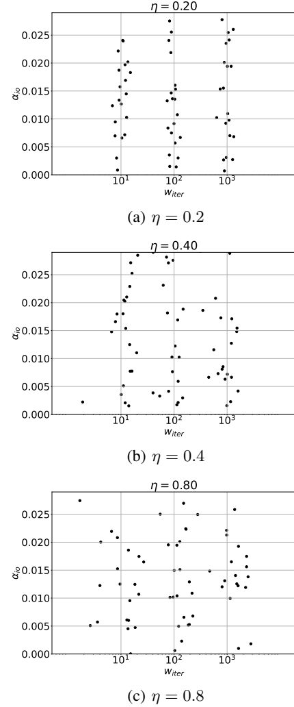
Figure 9: Workloads from Section VI-B1 : each dot represents characteristic time ( w_{\text{iter}} ) and I/O load ( \alpha_{\text{io}} ) for a job.
