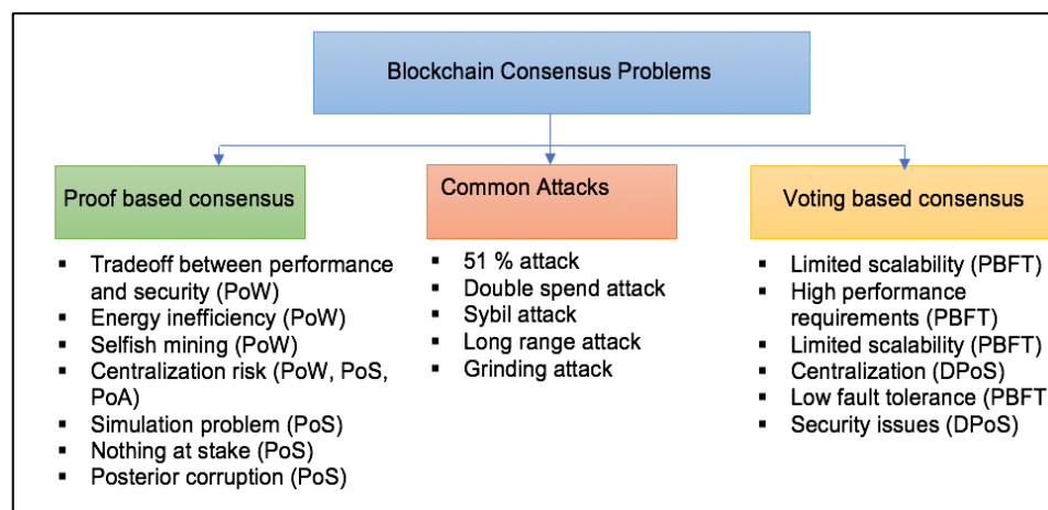
Figure 3: Blockchain consensus protocol challenges
