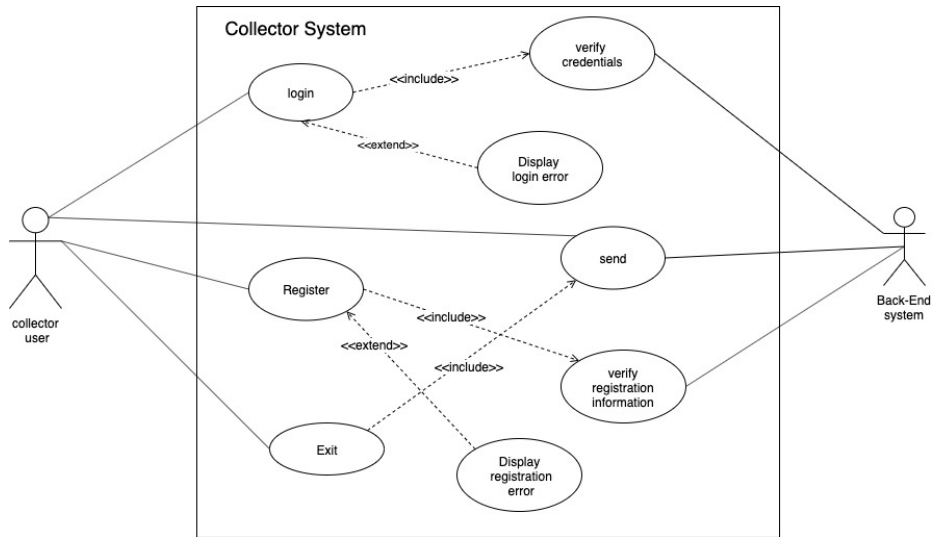
Fig. 1. Use case diagram for the collector
