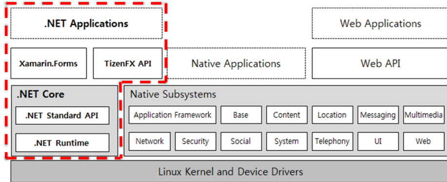
Fig. 1. Tizen .NET architecture
