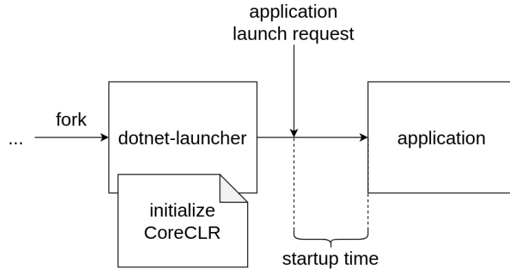
Fig. 2. CoreCLR initialization in candidate process
