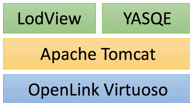
Fig. 4. LLOD publishing platform
