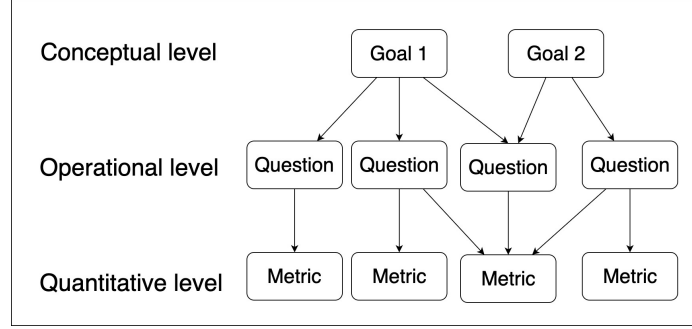
Fig. 1: Levels of the GQM model
