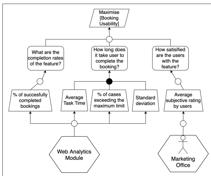
Fig. 6: Integrating GQM into the Goal model
