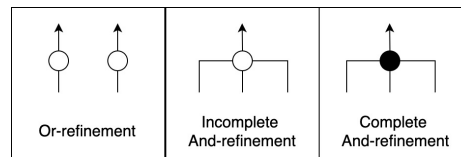
Fig. 3: Refinement types
