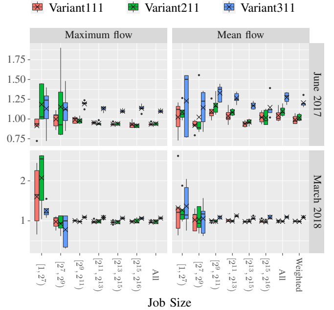
Figure 15: Maximum flow and mean flow relative to BASELINE for various timing decision (111: immediately interrupting, 211: proactive checkpointing, 311: waiting next checkpoint) and for various categories of job sizes. MTBF and downtime are both set to 1 hour.
