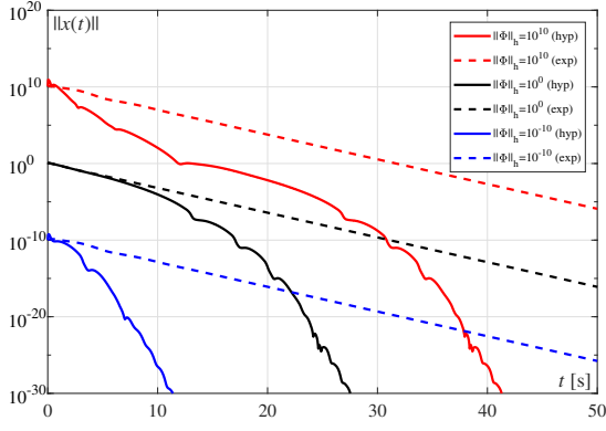
(a) Different initial conditions ( h = 1 [s])
