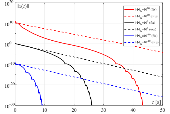
Fig. 2: Fixed-time (fix) vs. exponential (exp) stabilization of system (8), (9b)
