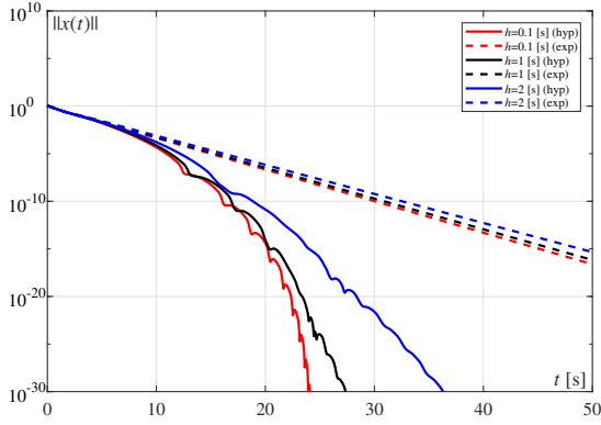
(b) Different time delays ( \|\Phi\|_h = 10^{10} )
